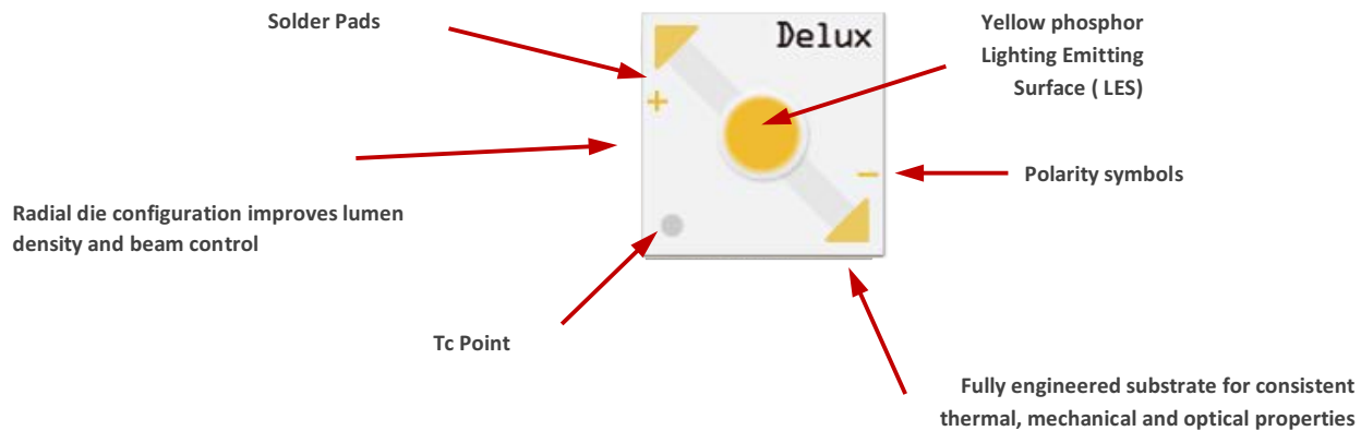
Figure 1: Array Features
